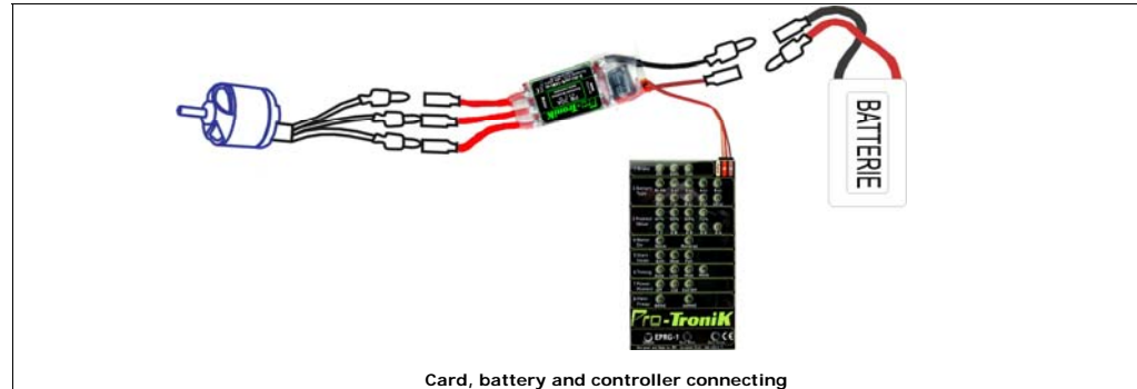
Card, battery and controller connecting
